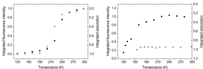
FIGURE 7.3. [Left] Temperature dependence of the absorption (circles) and fluorescence (squares) spectra of 1o in isopentane. The fluorescence spectra are integrated over the range 450–800 nm and subsequently the intensity at a given temperature is scaled relative to that at 298 K. Similarly, the absorption spectra were integrated over the interval 443–550 nm. A constant background was subtracted and the integrated spectra were scaled to that at 120 K. [Right] Integrated temperature dependent absorption spectra of 2o in ethanol (circles) and integrated temperature dependent fluorescence spectra of 2o in isopentane (squares).
